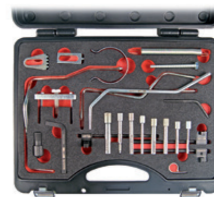
▶ BE507203 JGO CALADO DIESEL PSA • Citroen, Peugeot • Motores 1.4D, 1.5D, 1.6D, 1.9D, 2.0D
